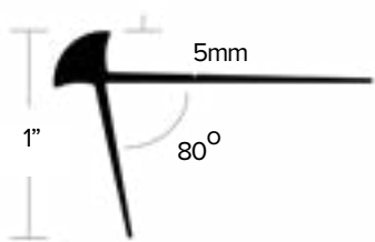
5MM NO-LIP STAIR NOSING 80° ANGLE
