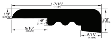
SQUARE NOSE (300)
