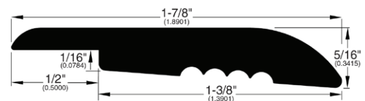
OVERLAP REDUCER (297)
