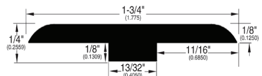
T-MOLD (299) *Fits up to 6mm floors
