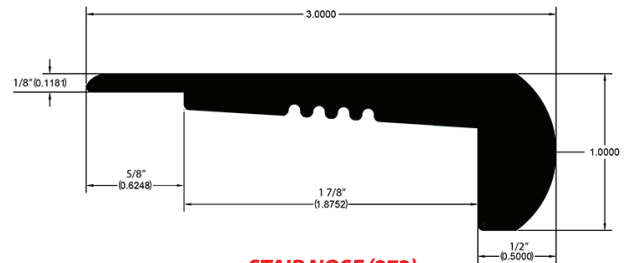
STAIR NOSE (273) *Fits up to 6mm floors
