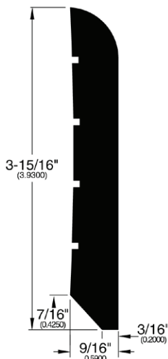
WALL BASE (294)
