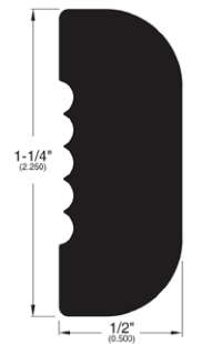
STAIR NOSE ADJUSTABLE (059)
