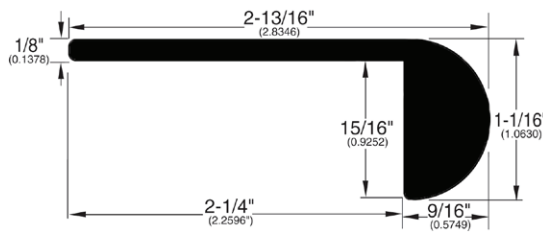
STAIR NOSE (298)
